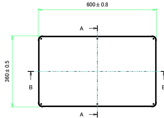
E view
